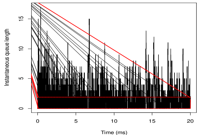
Fig 1: Traffic behavior of the true self-similar traffic over time
