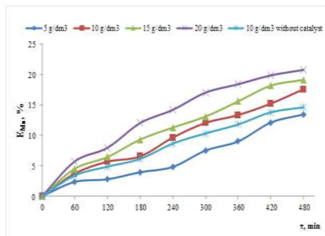
Figure 4- Degree of manganese extraction during leaching of mill tailings depending on the concentration of sulfuric acid in the presence of a paramagnetic catalyst
