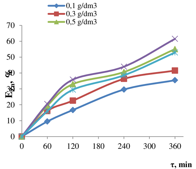
Figure 7 - Extraction of zinc from mill tailings at various concentrations of sodium cyanide in the presence of a paramagnetic catalyst
