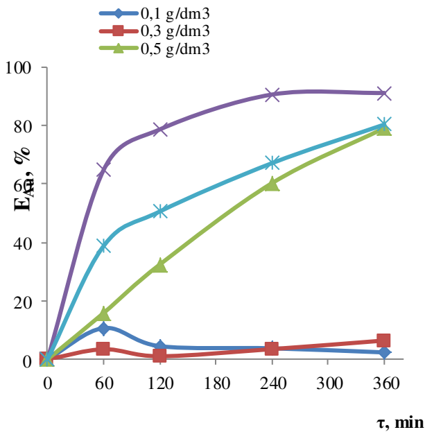
Figure 5 - The degree of gold extraction from mill tailings at different concentrations of sodium cyanide in the presence of a paramagnetic catalyst
