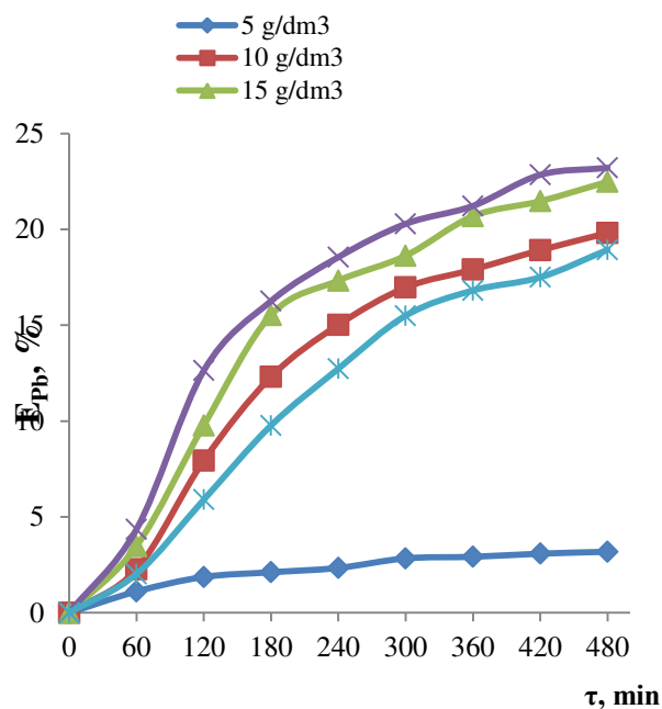
Figure 3 - Degree of extraction of lead during leaching of mill tailing depending on the concentration of sulfuric acid in the presence of a paramagnetic catalyst
