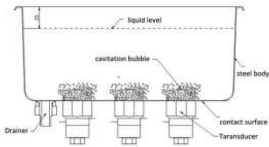
Figure 2 Schematic diagram of ultrasonic assisted Transesterification process
