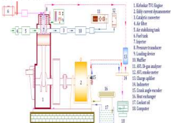
Figure 3. Schematic diagram of the experimental setup
