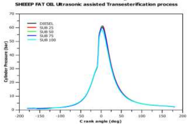
Figure 9. In-cylinder pressure against crank angle
