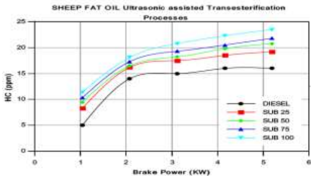
Figure 6. Hydrocarbon emission against brake power
