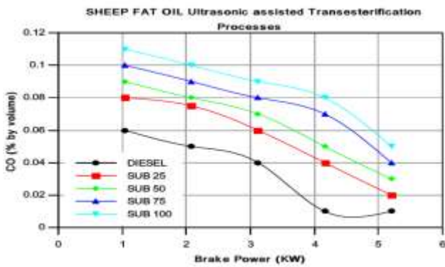
Figure 5. CO emission against Brake power
