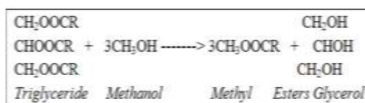
Figure 1 Transesterification process of converting Sheep fat oil to biodiesel
