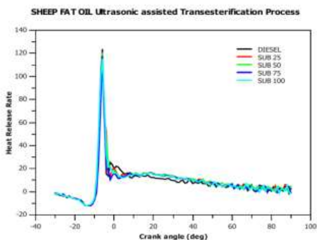
Figure 10. Heat release rate against crank angle
