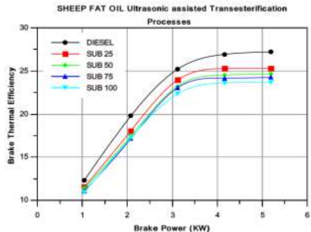
Figure 4. Brake thermal efficiency against brake power
