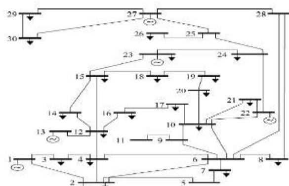
Fig 4.IEEE 30 bus system
