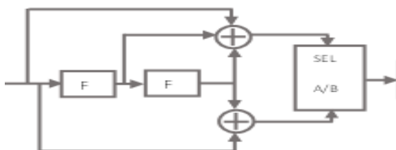
Fig.5. Code convolution structure rate \frac{1}{2} [4]
