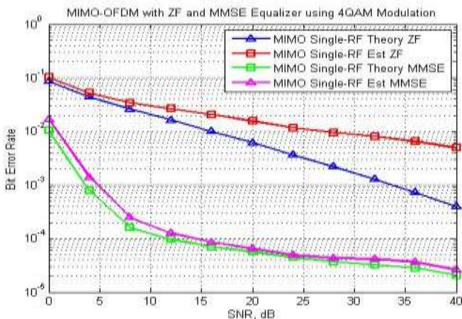
Fig. 9. BER performance of MIMO-OFDM system with ZF and MMSE equalizer using 4-QAM modulation
