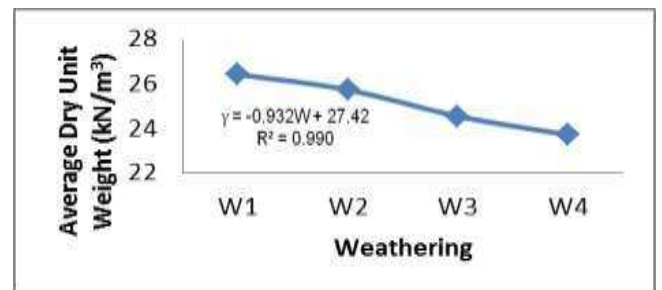
Figure 10: Average dry unit weight test results as a function of weathering states
