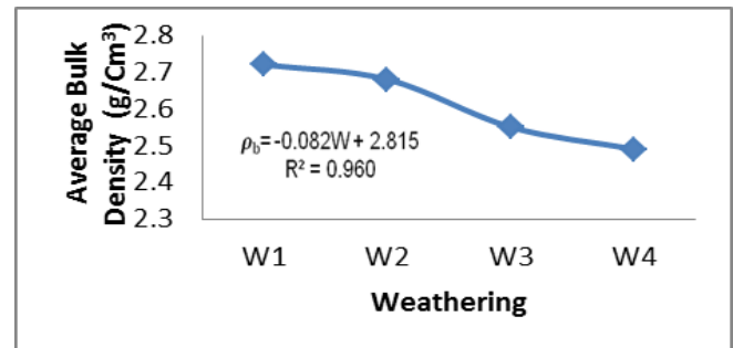
Figure 8: Average bulk density test results as a function of weathering states
