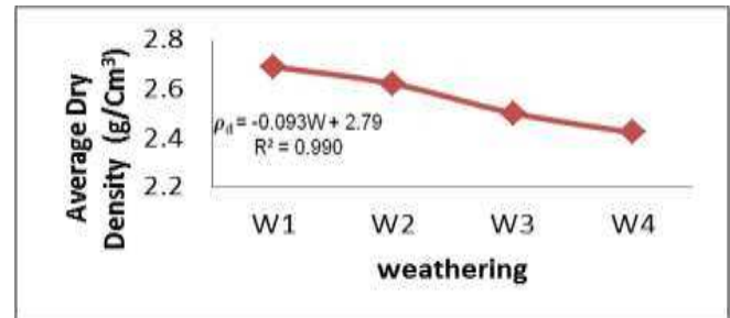
Figure 9: Average dry density test results as a function of weathering states
