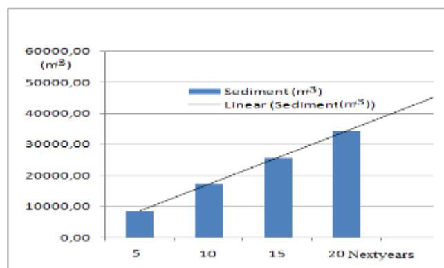
Fig. 6: The curve of growing of deposited material or expanded land to the offshore direction due to extra additional material sedimentation from mud volcano
