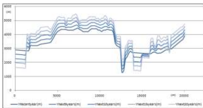
Fig. 4 the result of implementation model using Komar-Inman formulation
