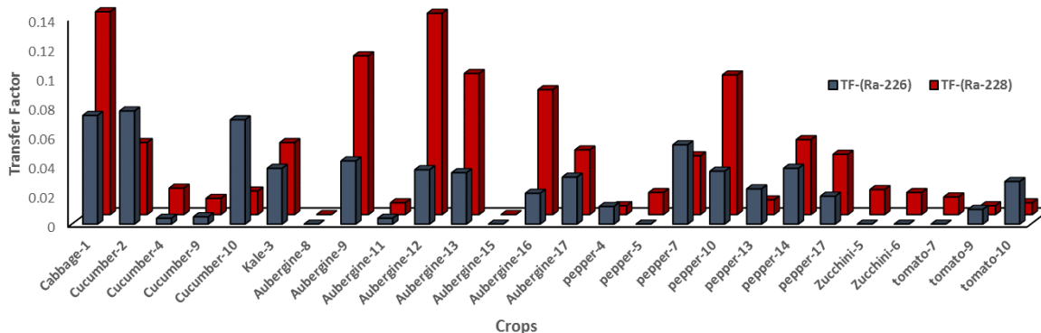
Figure 3. The transfer factors ( TF_s ) of ^{226}\text{Ra} and ^{228}\text{Ra} radionuclides in the crops at different locations
