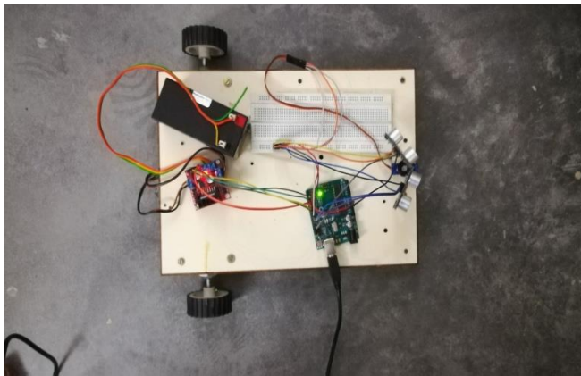
Fig.7. Final Prototype
