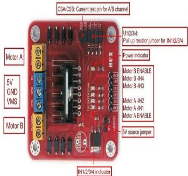
Fig.5. Motor Driver
