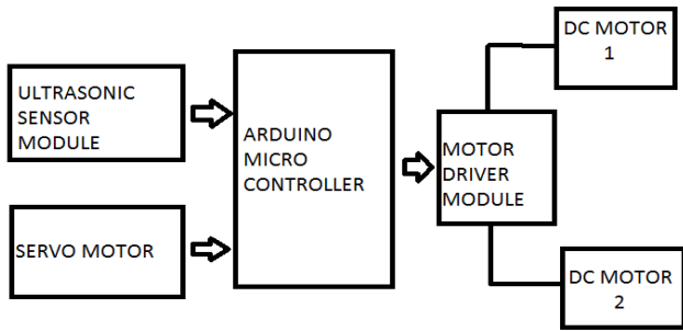
Fig.2.Architecture
