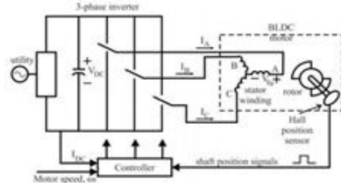
Figure 3: Electronically commutated BLDC motor drive.
