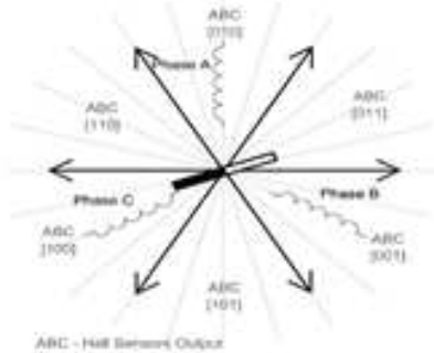
Figure 6 - Stator Flux Vectors at Six-Step Control.
