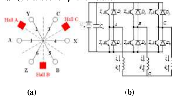
Figure 4-(a) Hall sensors position detection. (b) Six steps Control Strategy for 3phase BLDC motor
