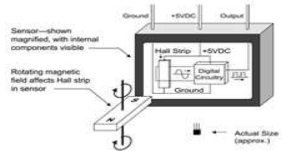
Figure 2: Hall effect sensor.
