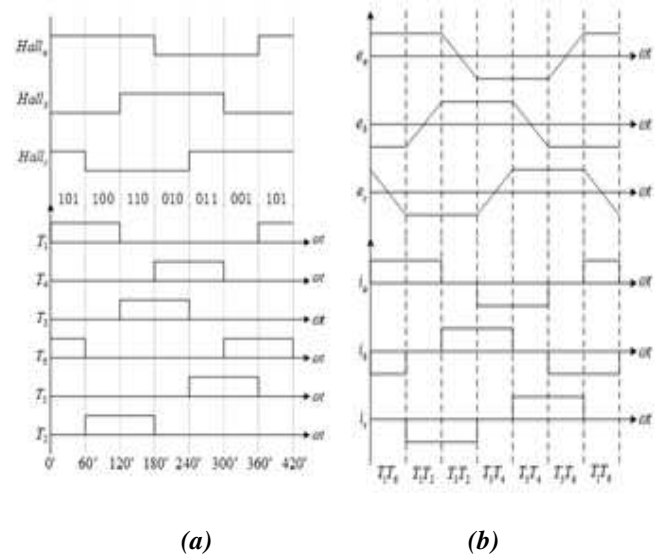
Figure 7- (a)Hall signal and inverter drive signals. (b)Three opposite potential and current waveforms.
