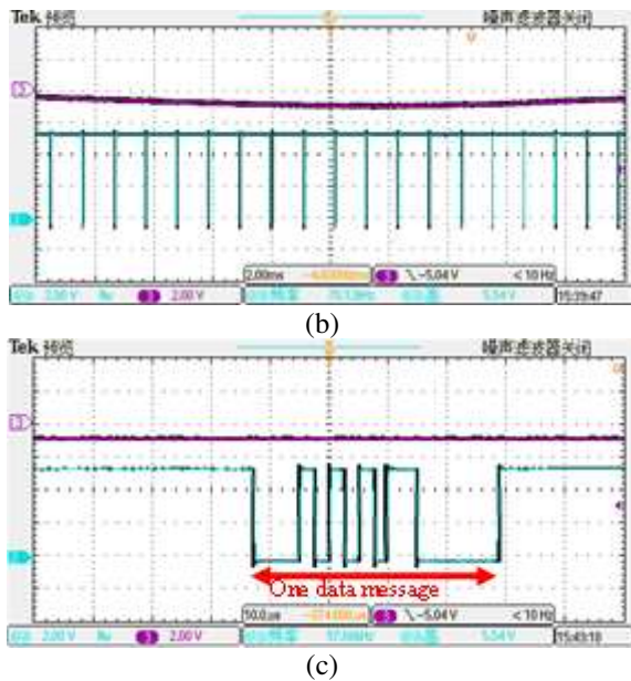
Figure 16 -(a), (b), (c): Experiment results of designed encoder by oscillograph. Angular position data vs time.
