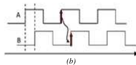
Figure 11. (a): B leads A CW rotation of the magnet and positive counting direction. (b): A leads B CCW rotation of the magnet and negative counting direction.
