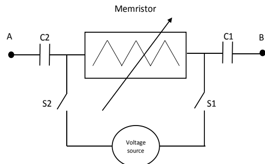
Fig. 4 Programmable resistor
