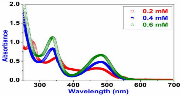
Figure 2. UV-VIS absorption spectrum of rifampin at different concentrations.
