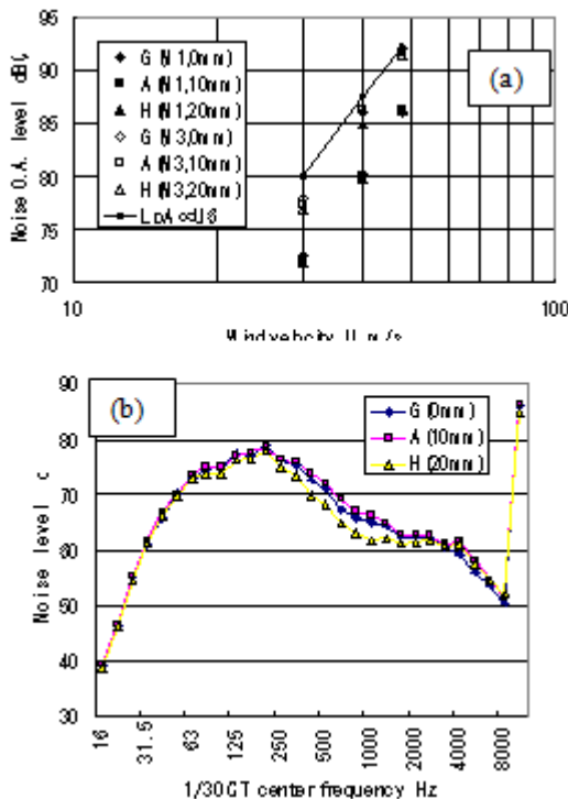
Fig.9 Effect of R of frame on noise level
