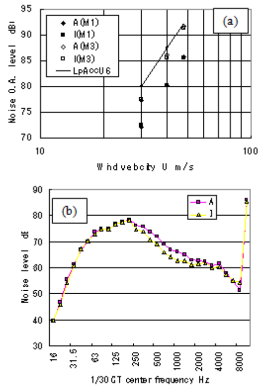
Fig.10 Effect of way of escape on noise level
