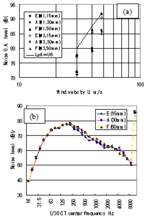
Fig.8 Effect of fin pitch on noise level
