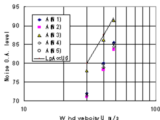
Fig.5 Noise level at each measuring point
