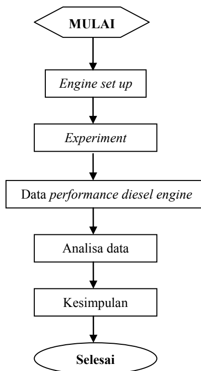
Gambar 1 Flowchart experiment
