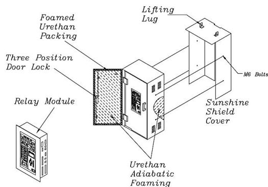
Gambar 2.6 Lay Out Kubikel Kontrol
