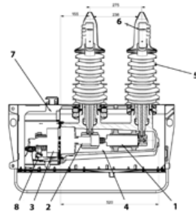
Gambar 2.1 Lay Out Recloser
