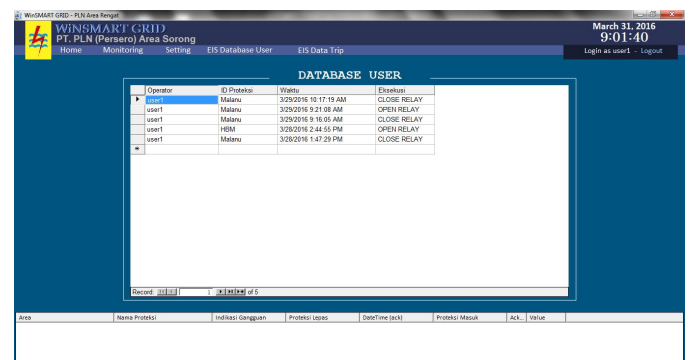
Gambar 3.10 Database User
