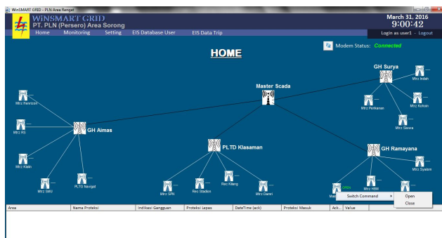
Gambar 3.7 Home
