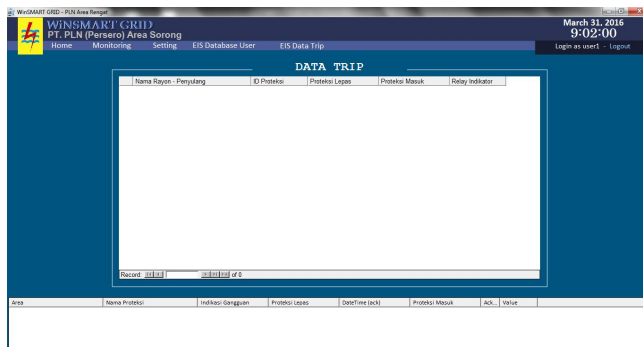
Gambar 3.11 Data Trip
