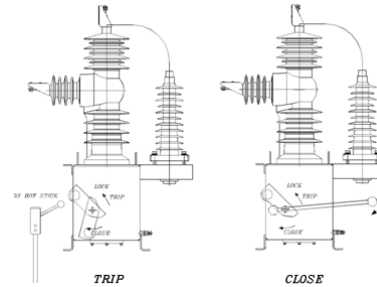
Gambar 2.5 Peralatan Manual Recloser/ Trip/ Closing/ Locking
