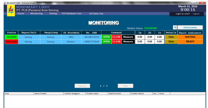
Gambar 3.3 Monitoring
