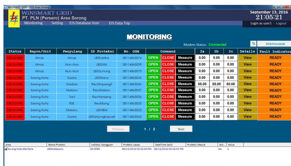
Gambar 3.13 Menu Monitoring
