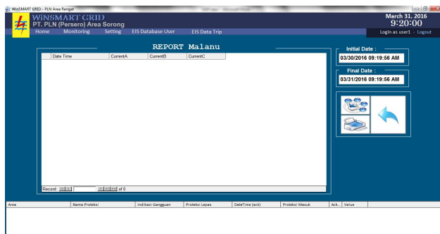
Gambar 3.6 Report
