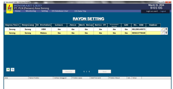
Gambar 3.8 Rayon Setting
