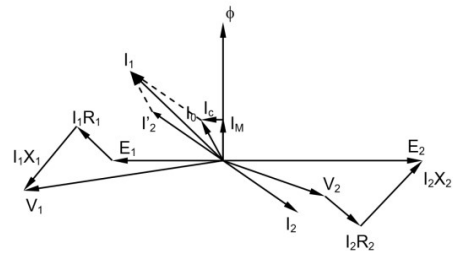
Gambar 2.4 Diagram Vektor 1
