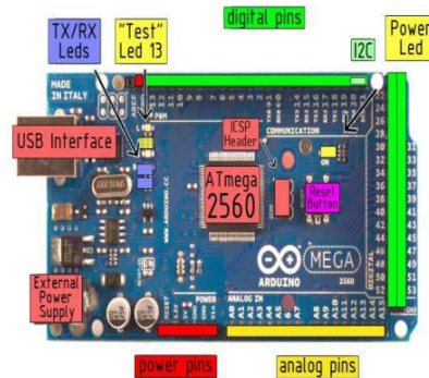
Sumber : ecadio.com/belajar-dan-mengenal-arduino-mega Gambar 2.2 Arduino MEGA2560 Rev3
