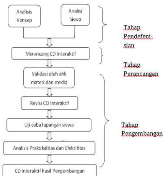
Gambar 2. Prosedur Penelitian
