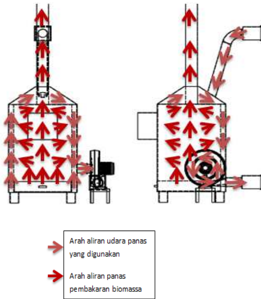
Gambar 5. Prinsip kerja Tungku Biomassa
