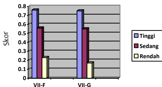
Gambar 2. Analisis N-Gain
