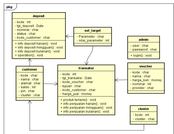
Gambar 8. Class diagram
