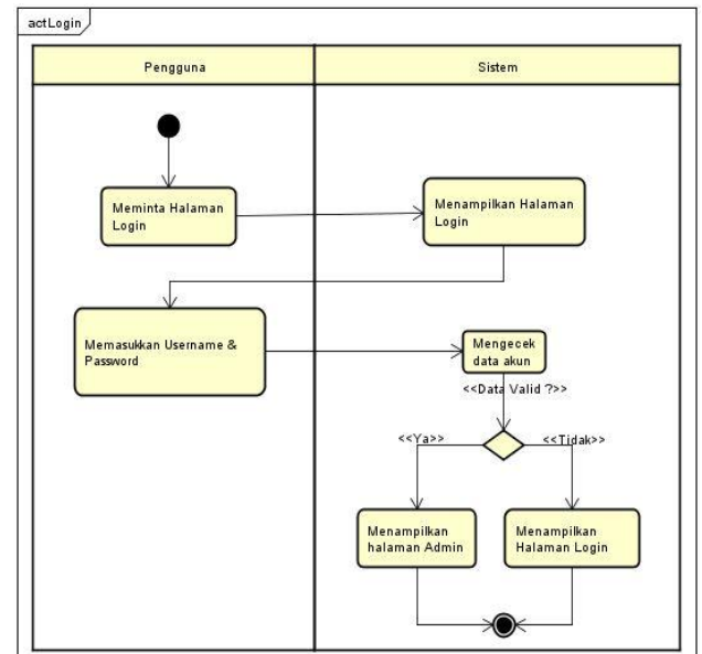
Gambar 4. Diagram Activity Login
