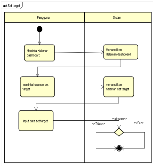
Gambar 6. Diagram Activity set target
