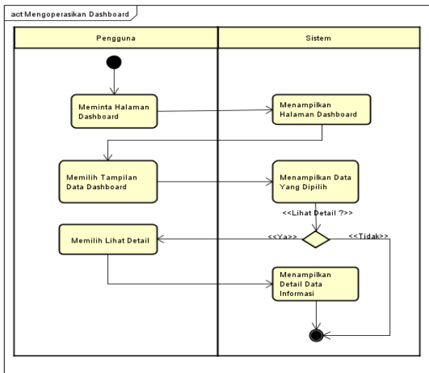
Gambar 5. Diagram Activity mengoprasikan Dashboard
