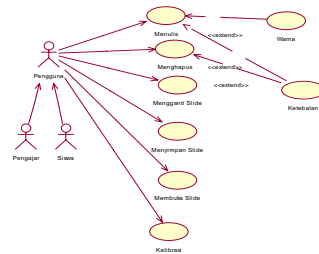
Gambar 3. Use Case Diagram Aplikasi Interactive Whiteboard
