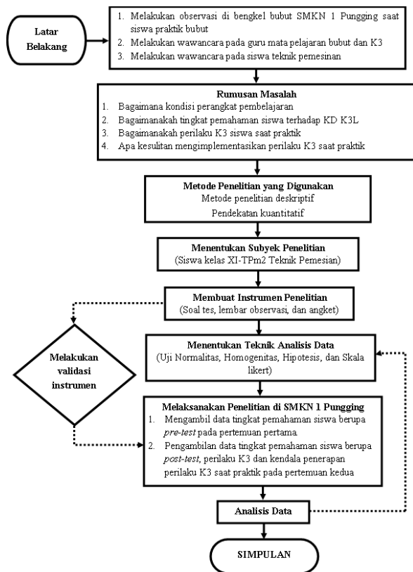
Gambar 2. Flowchart Penelitian
