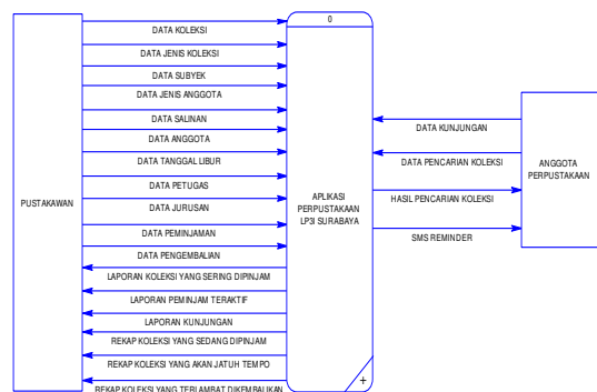
Gambar 6 Context Diagram
