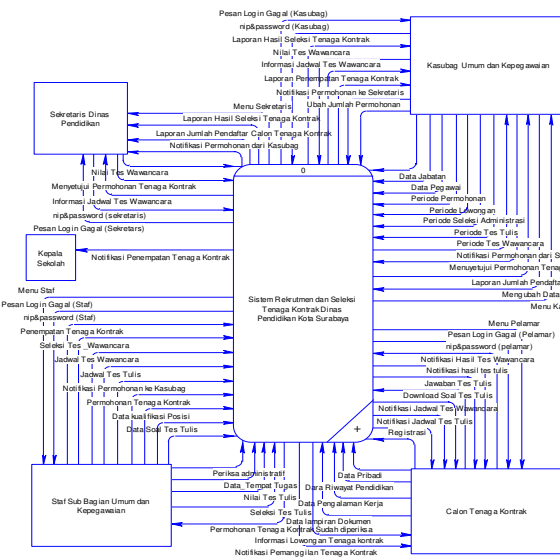
Gambar 1 DFD Level Context
