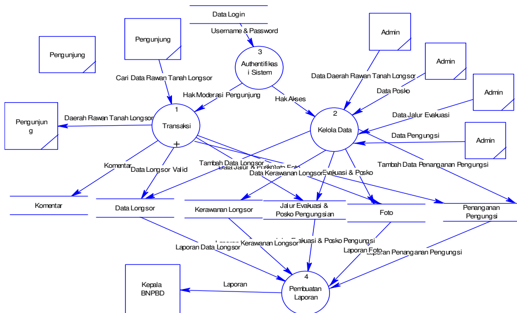
Gambar 3. DAD level 1
