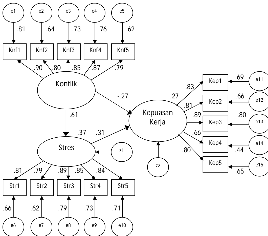
Gambar 1. Hasil Pengujian Structural Equation Modeling (SEM)
