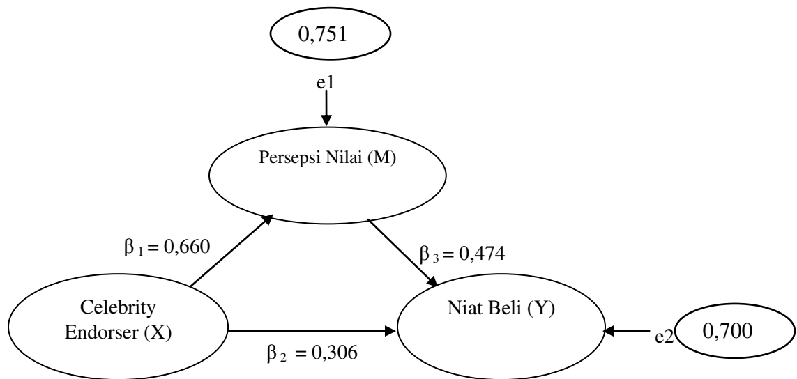
Gambar 2. Validasi Model Diagram Jalur
