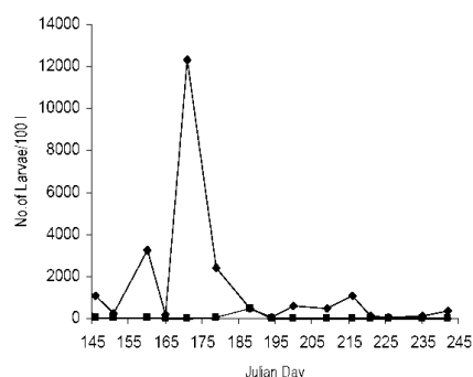
Figure 3. Densities of Quahog Larvae at Early and Late Stages in Warwick Pt.
