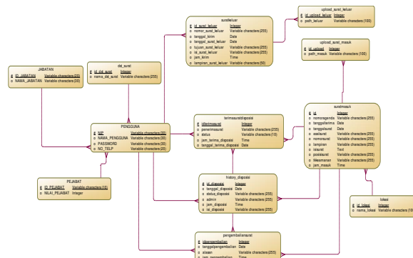
Gambar 3 Conceptual Data Model
