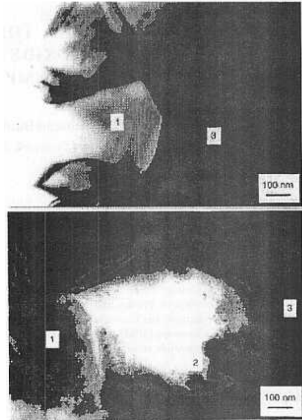
Figure 1a and b: Analytical Transmission Electron Microscopy Micrographs on Yttrium uncoated MA 956
