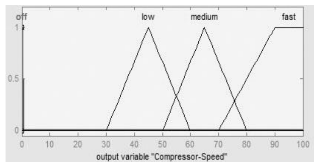
Figure 4. Compressor Speed Variable
