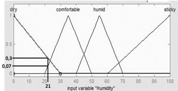
Figure 6. Humidity Fuzzification With Crisp Input 21%
