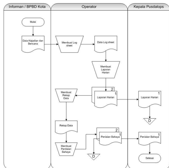
Gambar 3 Document Flow
