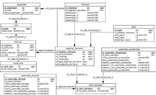
Gambar 9 PDM
