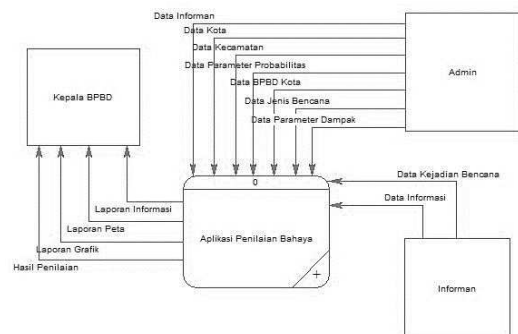
Gambar 6 Context Diagram
