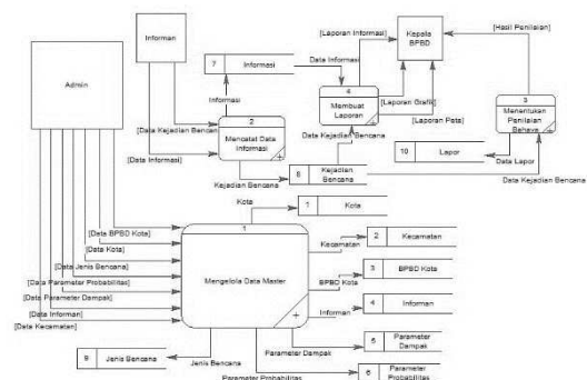
Gambar 7 DFD Level 0
