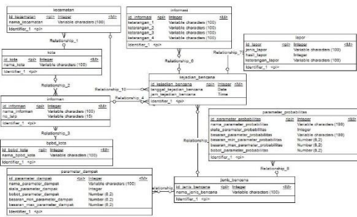
Gambar 8 CDM
