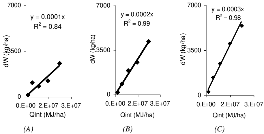
Figure 4. Light use efficiency of treatment: (A) control, (B) 7 mm day -1 and (C) 14 mm day -1 .
