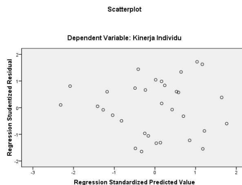
Gambar 1 Scatteplot
