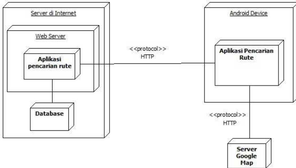
Gambar 3. Deployment Diagram
