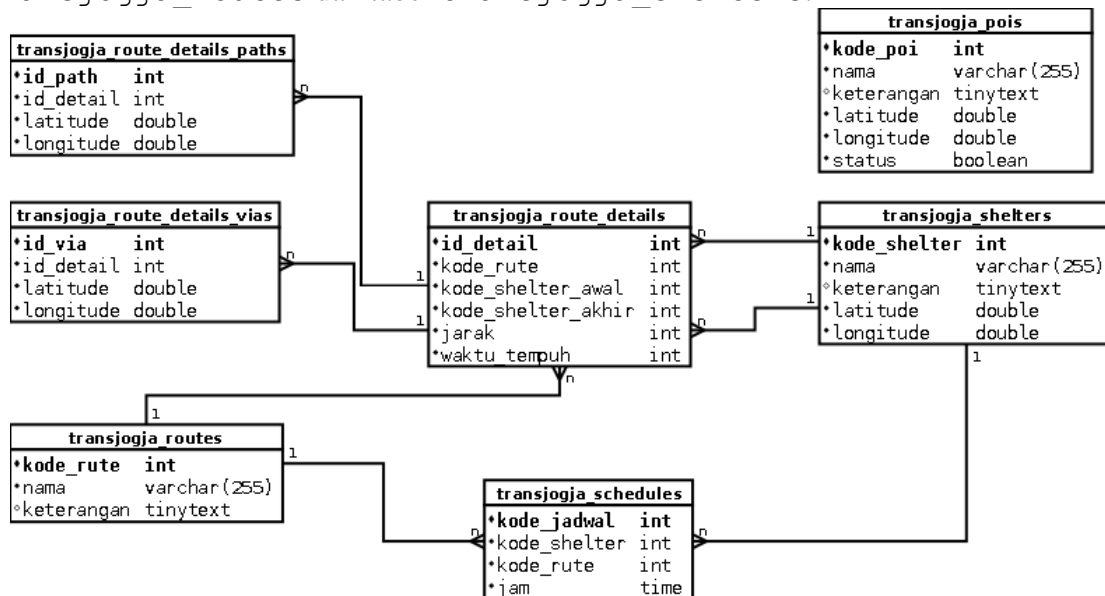
Gambar 4. Desain Basis Data
