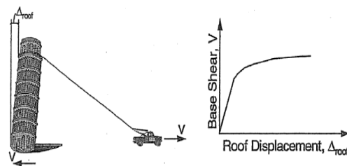
Fig. 1 Illustration of Pushover Analysis [ATC 40]
