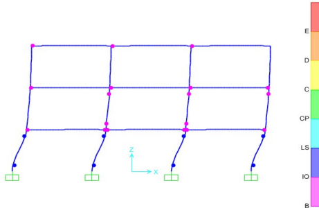
Fig. 12d Deformed Shape of the Frame-2 for Haql (X-Dir)
