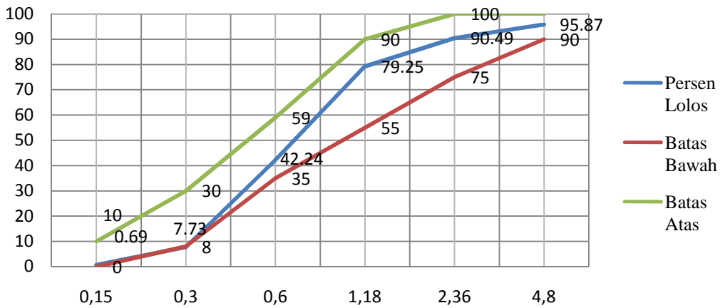
Gambar 2. Agregat Halus Zone 2 (Hasil Laboratorium)
