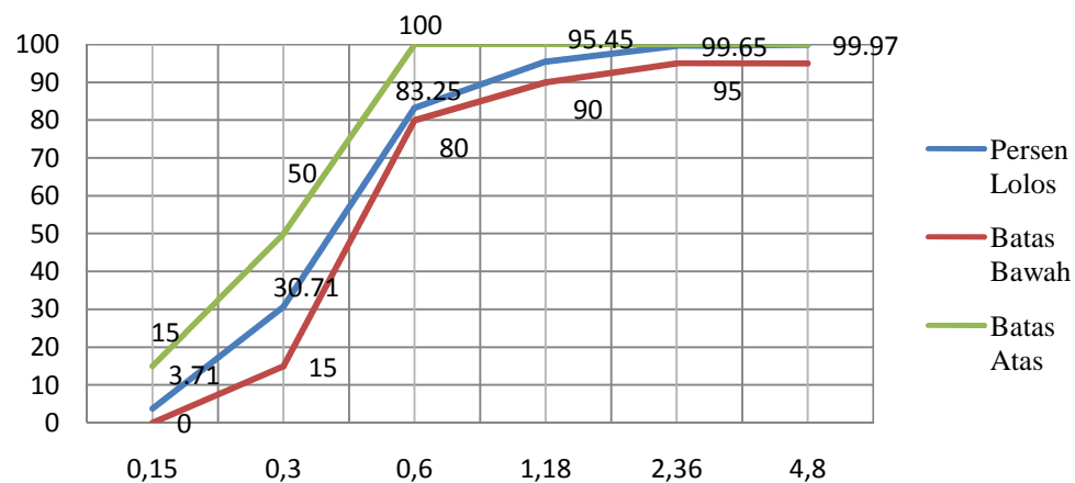
Gambar 4. Agregat Halus Zone 4 (Hasil Laboratorium)
