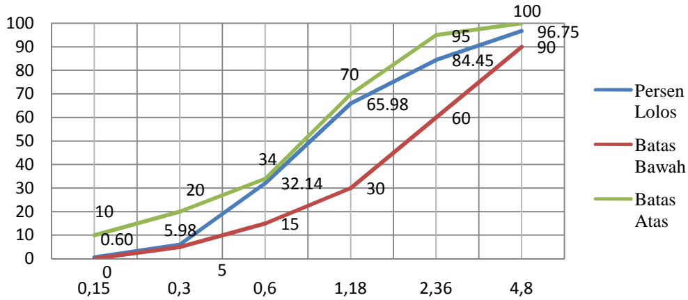
Gambar 1. Agregat Halus Zone 1 (Hasil Laboratorium)
