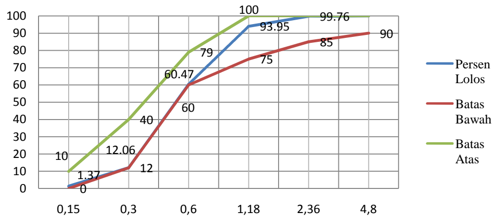
Gambar 3 Agregat Halus Zone 3 (Hasil Laboratorium)
