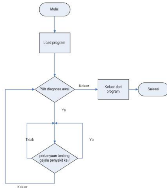
Gambar 6. Flowchart program
