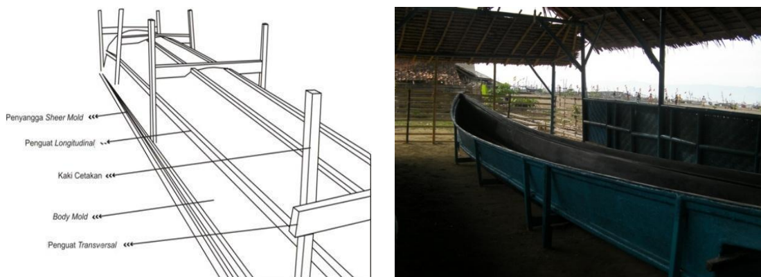
Gambar 1 Mold perahu fiberglass
