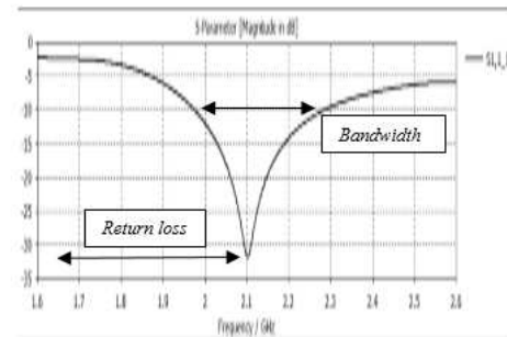
Figure 3.a. S-Parameter
