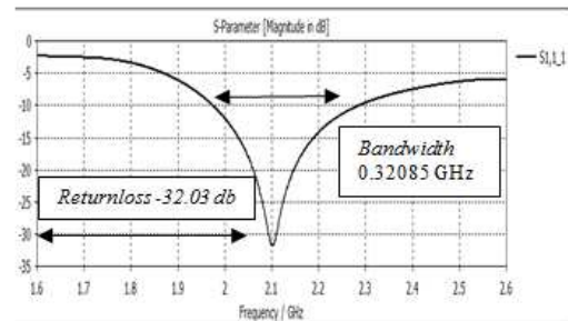
Figure 3.b. S-Parameter
