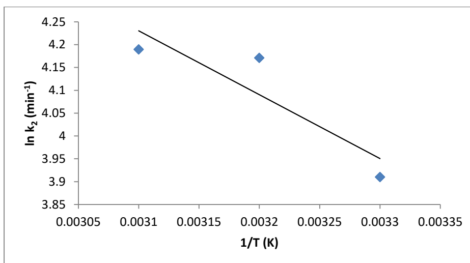
Fig.6: Temperature dependency of reaction rate
