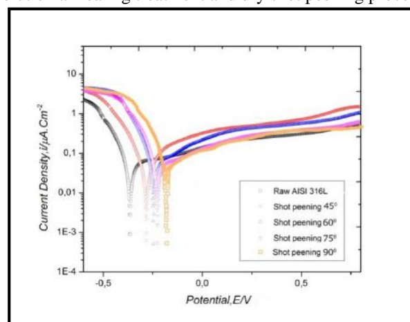
Fig.2: Result of Corrosion Test of the AISI 316L
