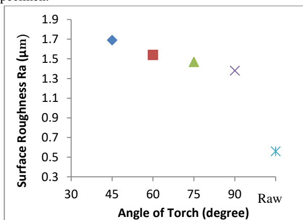
Fig.1: The Effect of Shot Angle To The Surface Roughness
