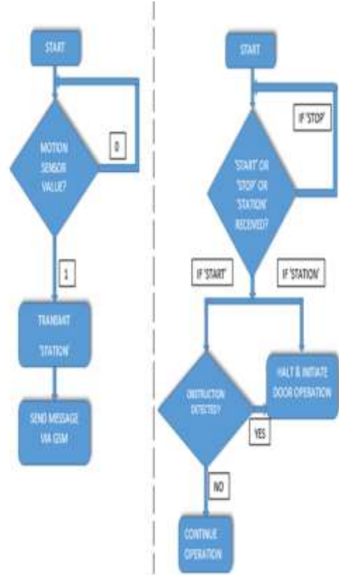
Fig.3. Flowchart of Automated Operation
