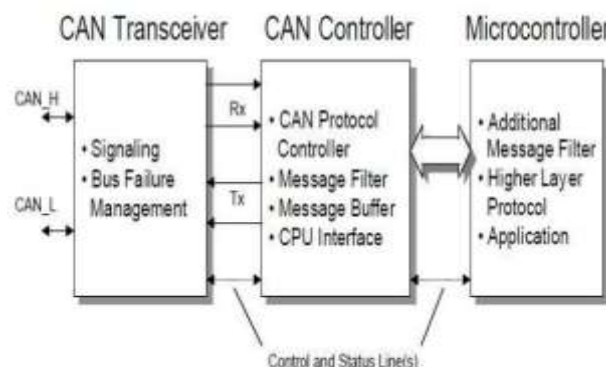
Fig.1: Can architecture
