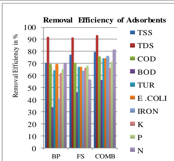
Chart.1: Removal Efficiency of Adsorbents
