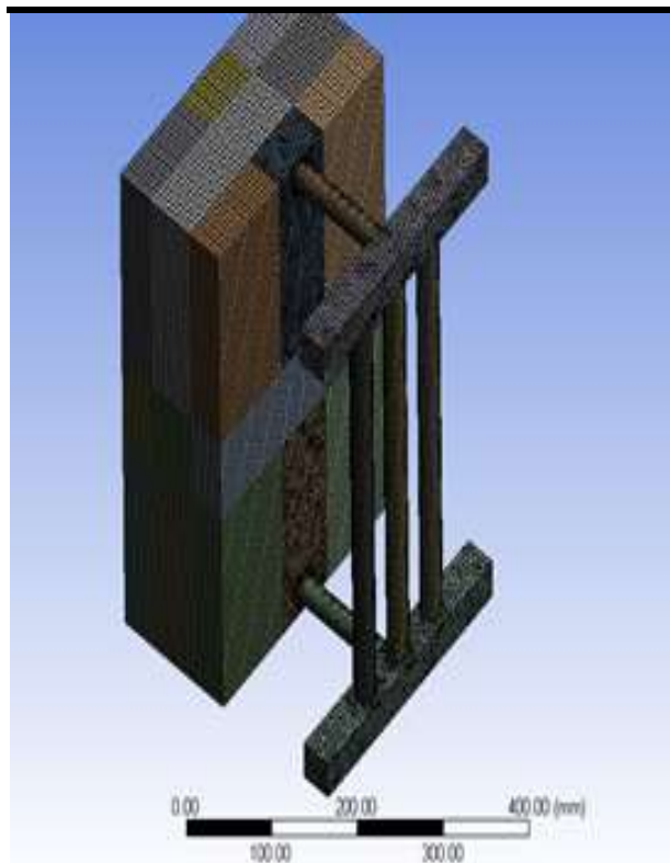
Fig 3: Meshed model
