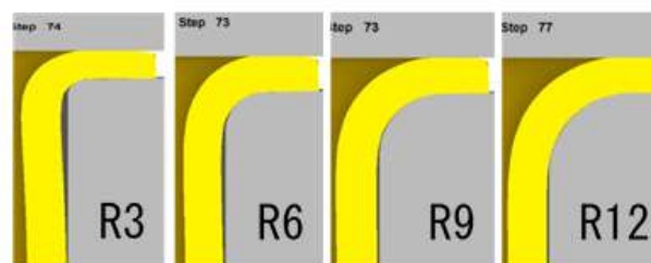
Fig.5: Analysis results of die corner R3 mm, R6 mm, R9mm and R12 mm
