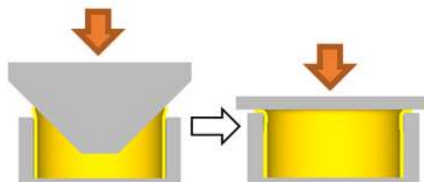
Fig.1: Schematic illustrations of analysis model of cold flaring process
