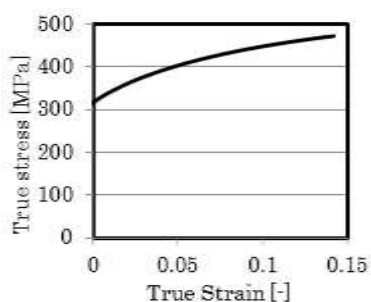
Fig.3: Flow stress of SGP pipe
