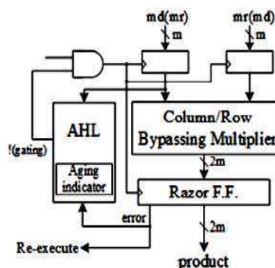
Fig. 8. Proposed architecture ( md means multiplicand; mr means multiplier).
