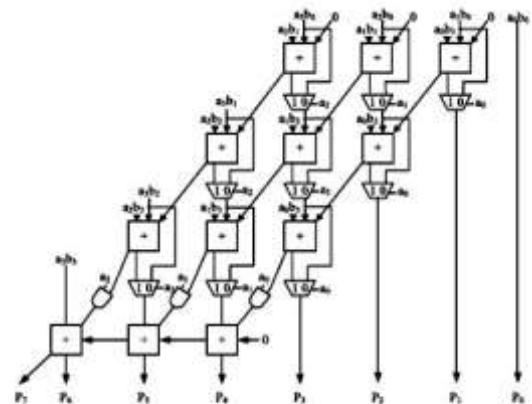
Fig. 2. 4 × 4 column-bypassing multiplier.
