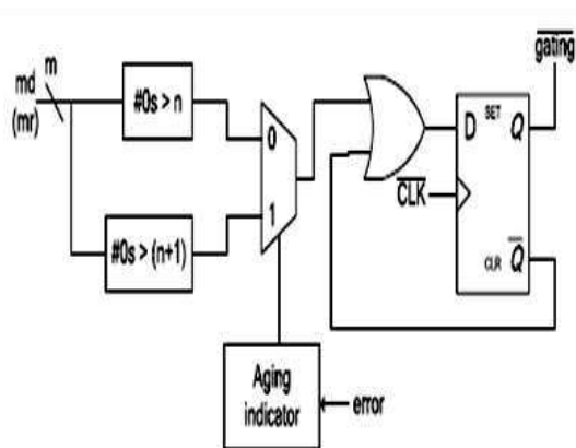
Fig. 12. Diagram of AHL (md means multiplicand; mr means multiplier).
