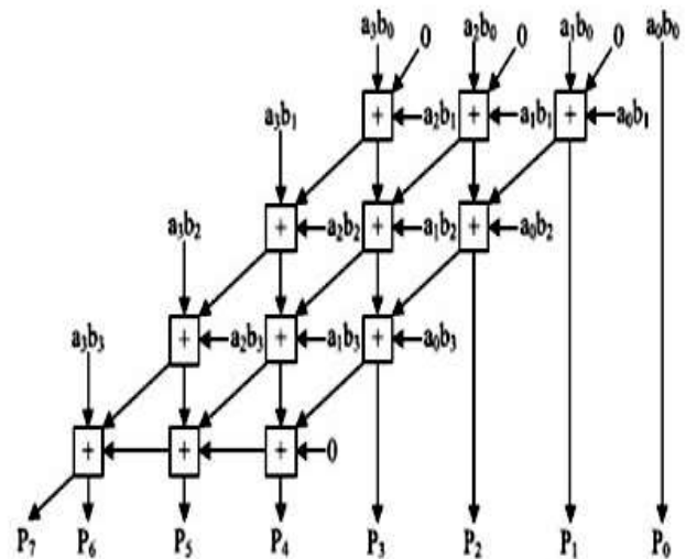
Fig. 1. 4 × 4 normal AM.
