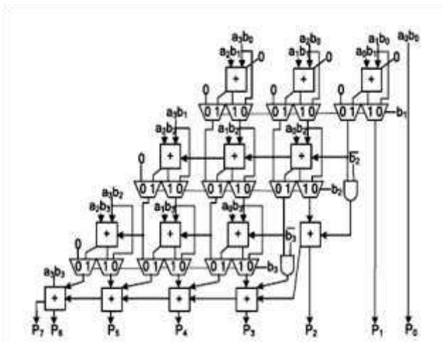
Fig. 3. 4 \times 4 row-bypassing multiplier.
