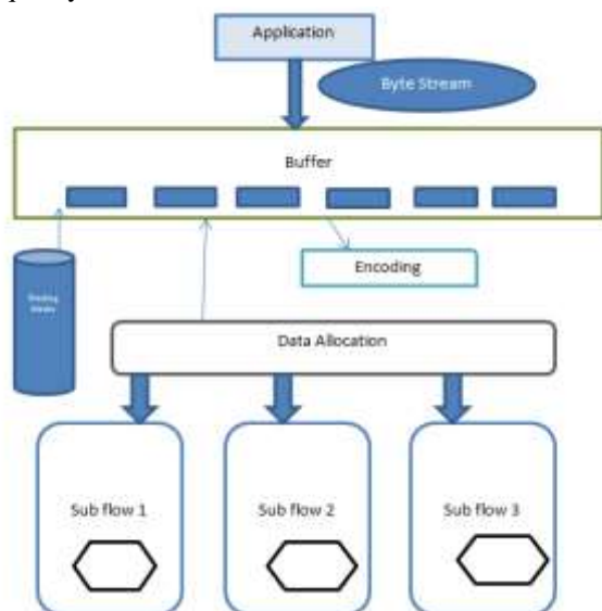
Fig.1.2: FMTCP Architecture.
